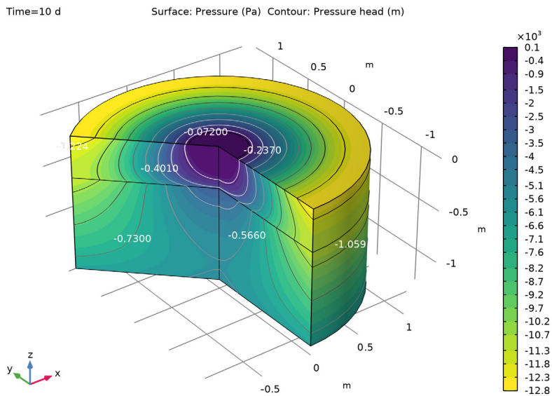
Figure 5: Pressure (surface plot), and pressure head (contours) distribution in a revolved geometry after 10 days.
