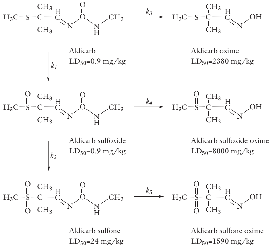
Figure 2: Reaction pathways of aldicarb degradation. The toxicity is indicated by its \text{LD}_{50} value (mg/kg), signifying the median lethal dose.
