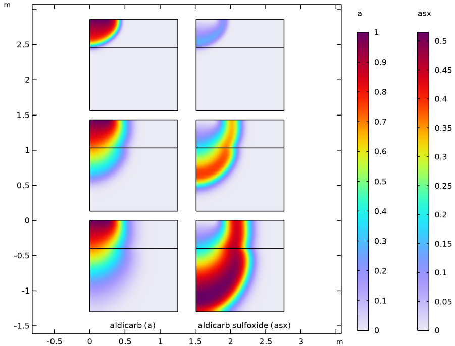
Figure 7: Concentration of aldicarb (left) and aldicarb sulfoxide (right) after 1 day (top), 5 days (middle), and 10 days (bottom).
