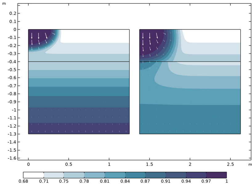
Figure 6: The effective saturation (surface plot) and flow velocity (arrows) in a variably saturated soil after 0.3 days (left) and 1 day (right).
