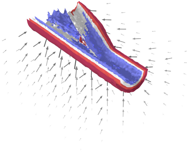
Isosurface plot of the fail function and Darcy velocity field (arrows) calculated from a poroelastic model for the branching junction in a multilateral well.
