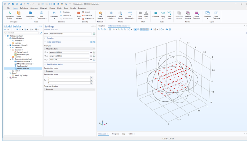
Figure 3-6: Graphics window after clicking the Preview Initial Coordinates button.
