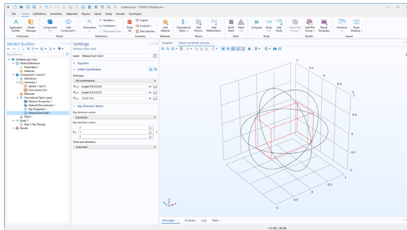
Figure 3-7: Graphics window after clicking the Preview Initial Extents button.
