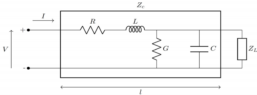
Figure 4-9: Schematic of a transmission line with a load impedance.
