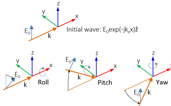
Figure 4-7: Schematic of the directions for the wave vector \mathbf{k} , the electric field \mathbf{E}_0 , and the roll, pitch, and yaw rotations. The top image represents an initial wave propagating in the x direction with a polarization along the z direction.
