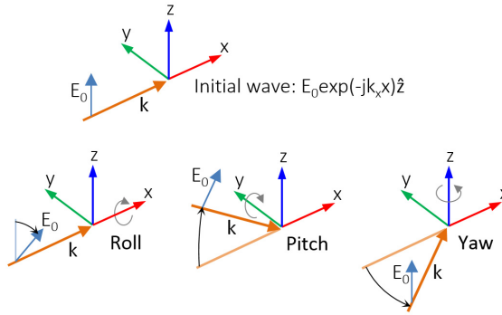
Figure 4-1: Schematic of the directions for the wave vector \mathbf{k} , the electric field \mathbf{E}_0 , and the roll, pitch, and yaw rotations. The top image represents an initial wave propagating in the x direction with a polarization along the z direction.
