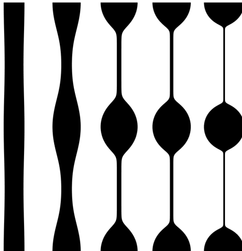
Figure 10: Filament profiles at 5 different dimensionless times: 0, 20, 30, 100, and 300.
