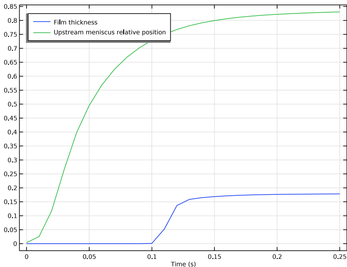
Figure 9: Film thickness and upstream meniscus position as a function of time.
