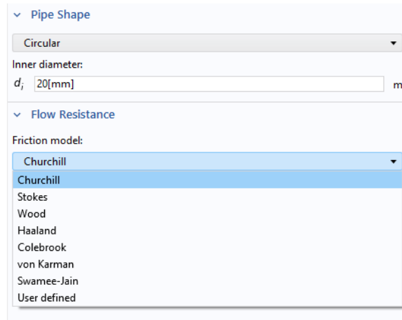
Figure 11: Select a shape and different predefined friction models in the Pipe Properties node.
