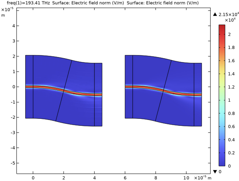
Figure 4: The electric field norms computed by the Electromagnetic Waves, Beam Envelopes (left) and the Electromagnetic Waves, Frequency Domain (right) interfaces, respectively.
