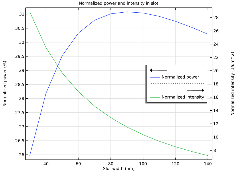
Figure 5: Normalized optical power and optical intensity through the slot with respect to the slot width for an operating wavelength of 1.55 μm.
