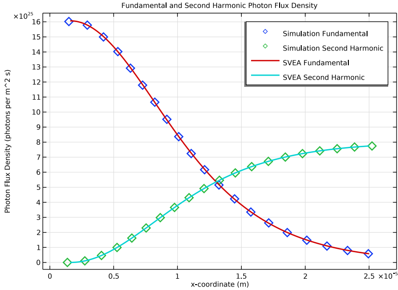
Figure 4: The photon flux density (in units of photons per m^2 and s ) for the fundamental and the second harmonic wave. The diamonds represent the simulated results (blue diamonds representing the fundamental wave and green diamonds representing the second harmonic wave), whereas the red line represents the analytical result in Equation 3 and the cyan line represents the analytical results in Equation 4.
