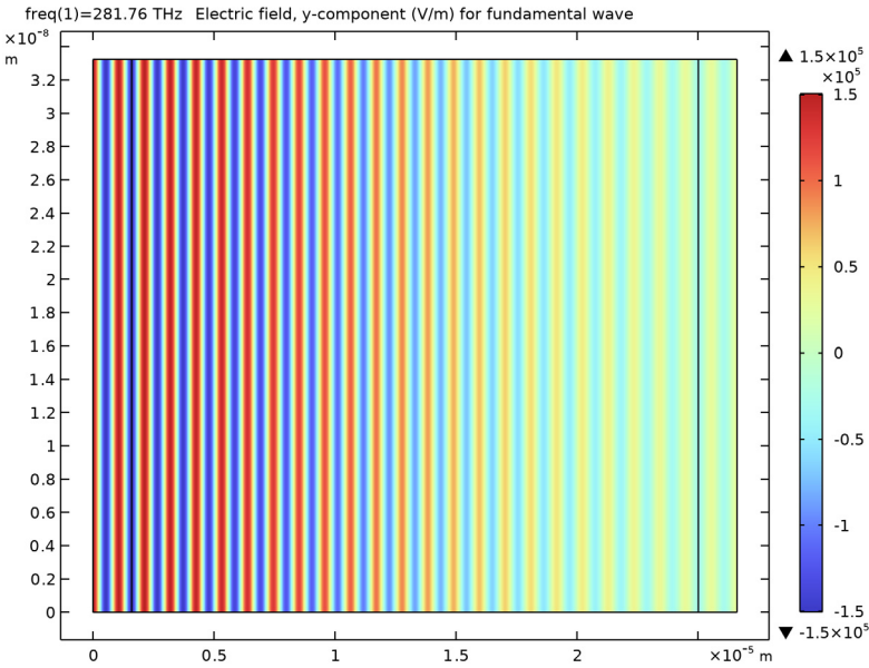
Figure 1: The electric field distribution of the fundamental wave (y-component).
