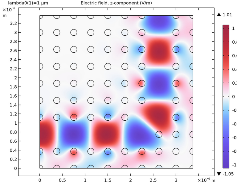
Figure 1: The z -component of the electric field showing how the wave propagates along the path defined by the pillars.
