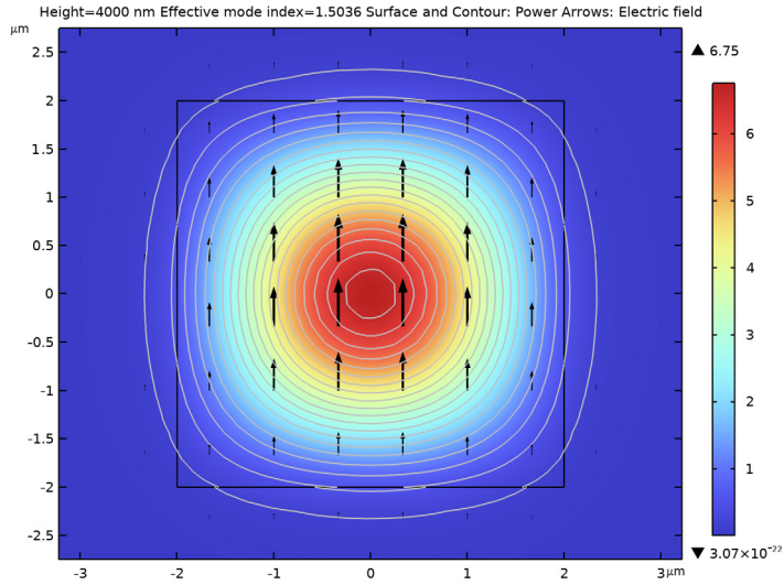
Figure 1: The power in the propagation direction (out-of-plane) for the dominant mode, E^y_{11} . The arrows show that the mode is polarized in the y direction.
