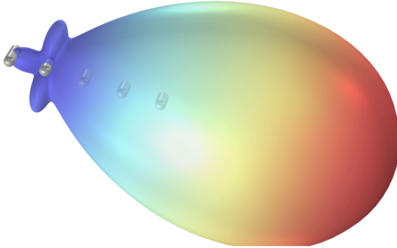
Figure 3: Far-field radiation pattern of the optical Yagi-Uda antenna, showing a high directivity.
