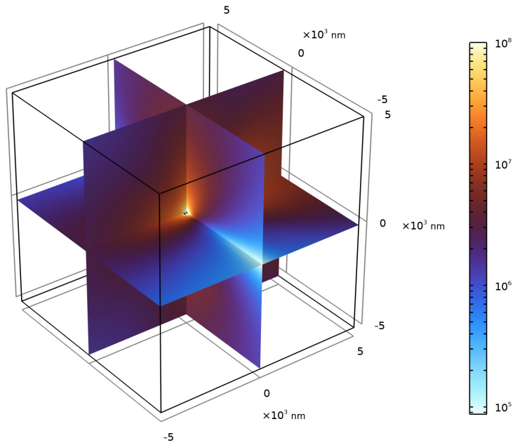
Figure 2: Norm of the electric field around the optical Yagi-Uda antenna. Using the Grid 3D dataset, we can evaluate the field quantities at arbitrary locations.
