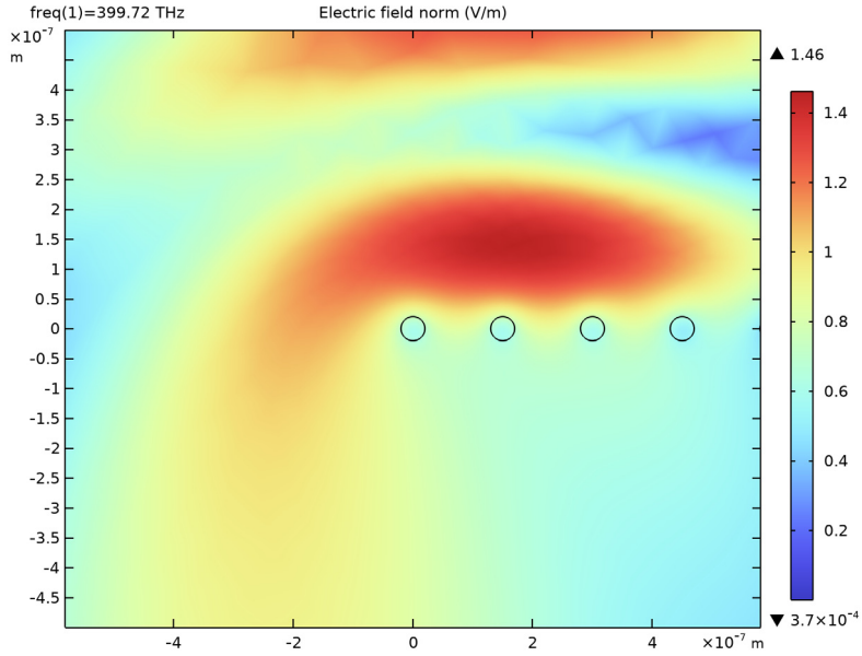
Figure 5: Zoom-in of the electric field norm for the center of the Gaussian beam and the leftmost nanorods. The Gaussian light beam is polarized along the rods (out-of-plane in the z direction).
