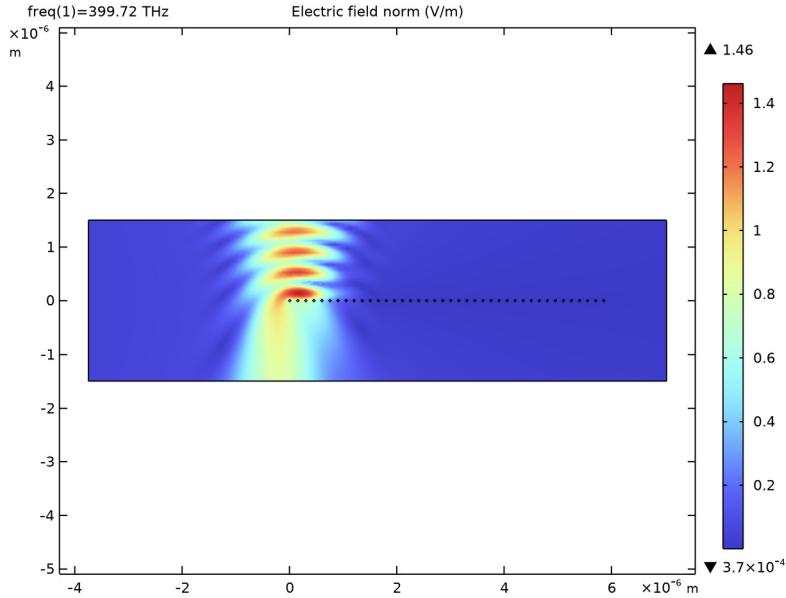
Figure 6: Surface plot of the full Gaussian beam and all the nanorods. The beam is polarized in the out-of-plane ( z ) direction.
