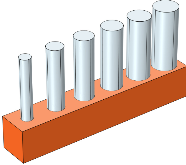
Figure 2: 1\ \mu\text{m} tall silicon posts on a \text{SiO}_2 substrate. The periodicity of the individual elements is 500\ \text{nm} , and so the full structure of six elements is 3\ \mu\text{m} wide.
