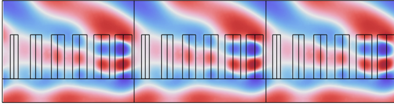
Figure 3: The electric field in the y direction for an array of 3 unit cells. Notice that the electric field wavefronts at the bottom of the structure are approximately horizontal, while the wavefronts at the top have been deflected to the right at approximately 31 degrees.
