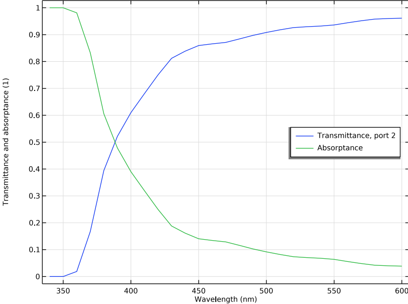
Figure 3: A plot of the transmittance and absorbance versus wavelength.
