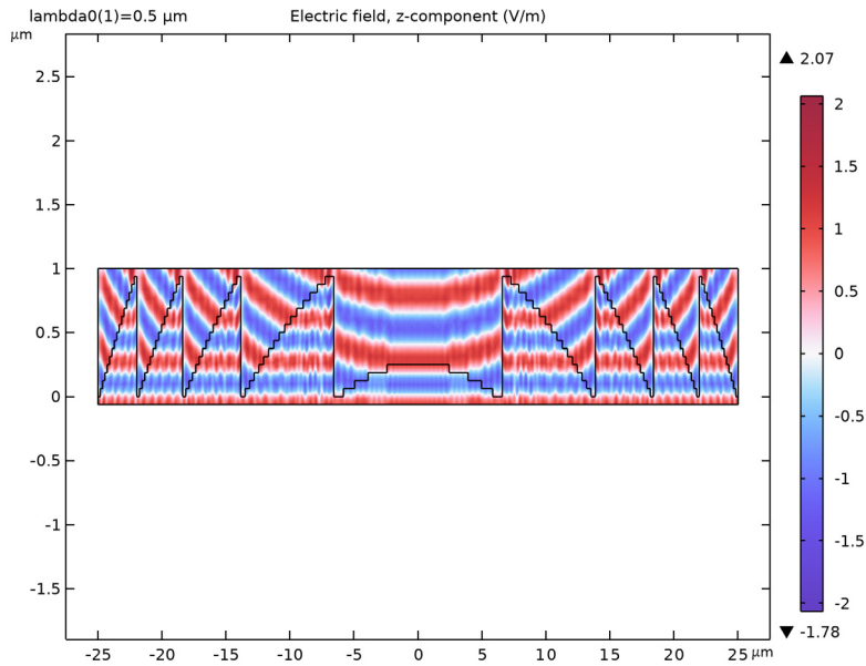
Figure 2: Electric field amplitude around the Fresnel lens. The plot is scaled as x:y = 1:10 .
