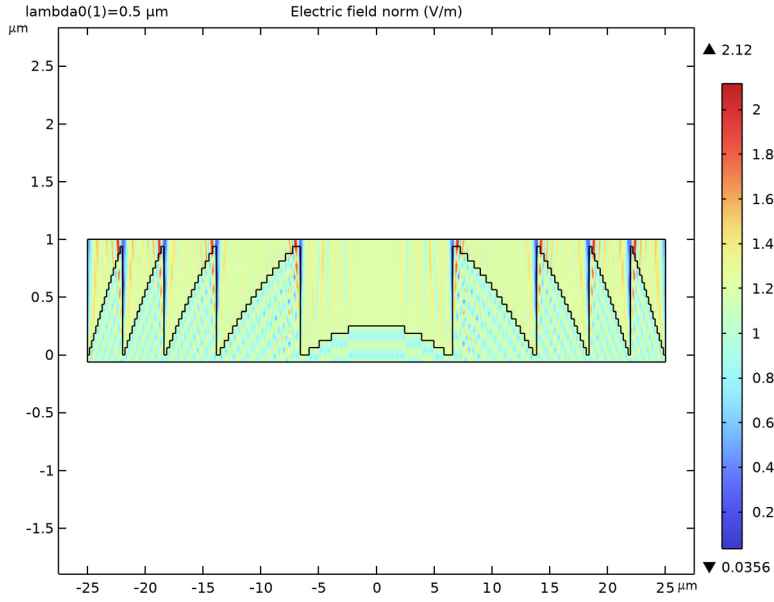
Figure 3: Electric field norm around the Fresnel lens. The plot is scaled as x:y = 1:10 .
