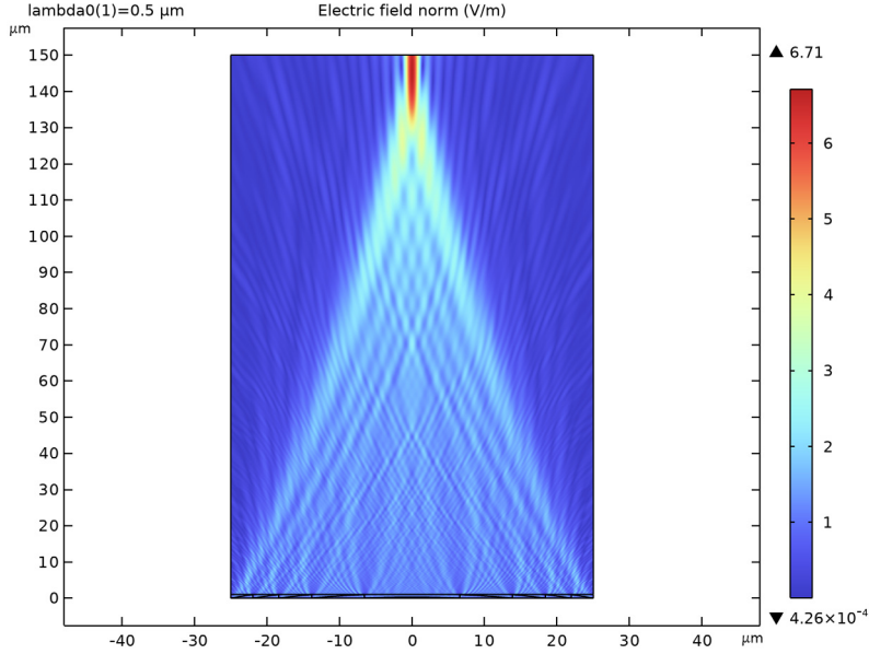
Figure 5: Electric field norm in the air domain. Note that the plot is scaled as x:y = 2:1 .
