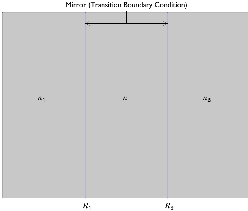
Figure 2: A mirror modeled as a thin dielectric layer with refractive index n , surrounded by materials with refractive indices n_1 and n_2 , respectively. The reflectances R_1 and R_2 , for each interface, are indicated at the bottom of the picture. Each mirror is modeled using a Transition Boundary Condition feature.
