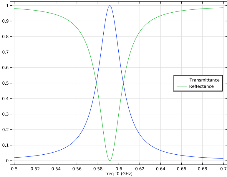
Figure 5: A frequency sweep over the resonance peak.
