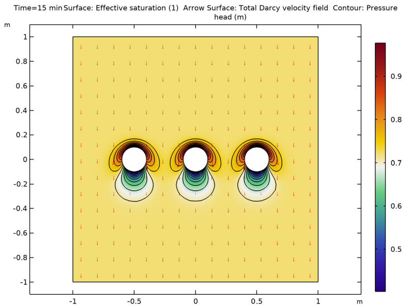
Figure 3: Solution for effective saturation (surface plot), pressure head (contours), and velocity (arrows) at 15 minutes for Soil Type I (van Genuchten).
