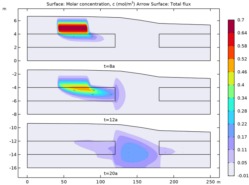
Figure 5: Solute concentration after 8, 12, and 20 years, displayed in one array.
