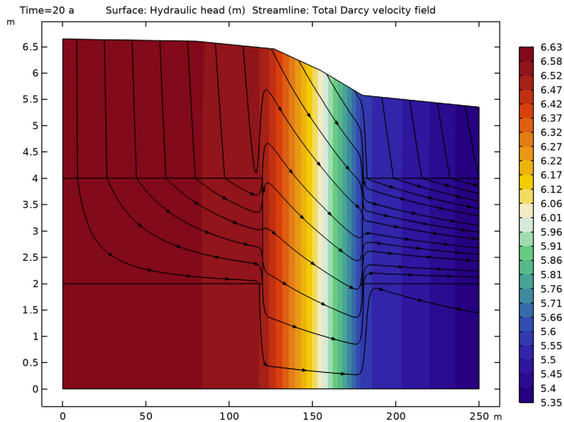
Figure 3: Estimated hydraulic head and flow lines.
