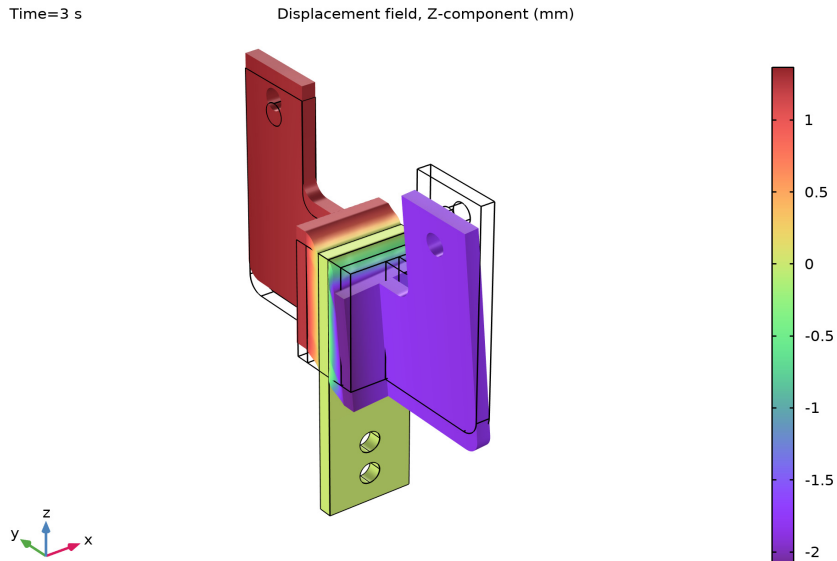
Figure 2: Displacement field.
