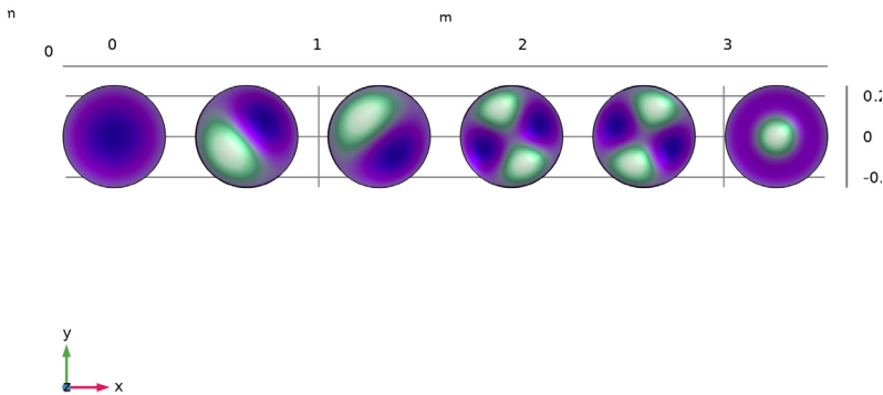
Figure 1: First six eigenmodes of the prestressed membrane.
