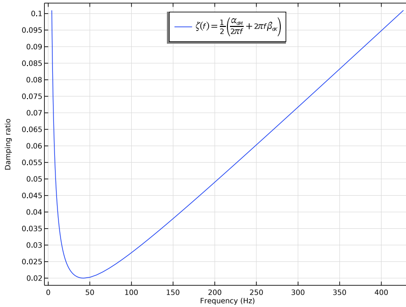
Figure 1: The damping ratio curve.
