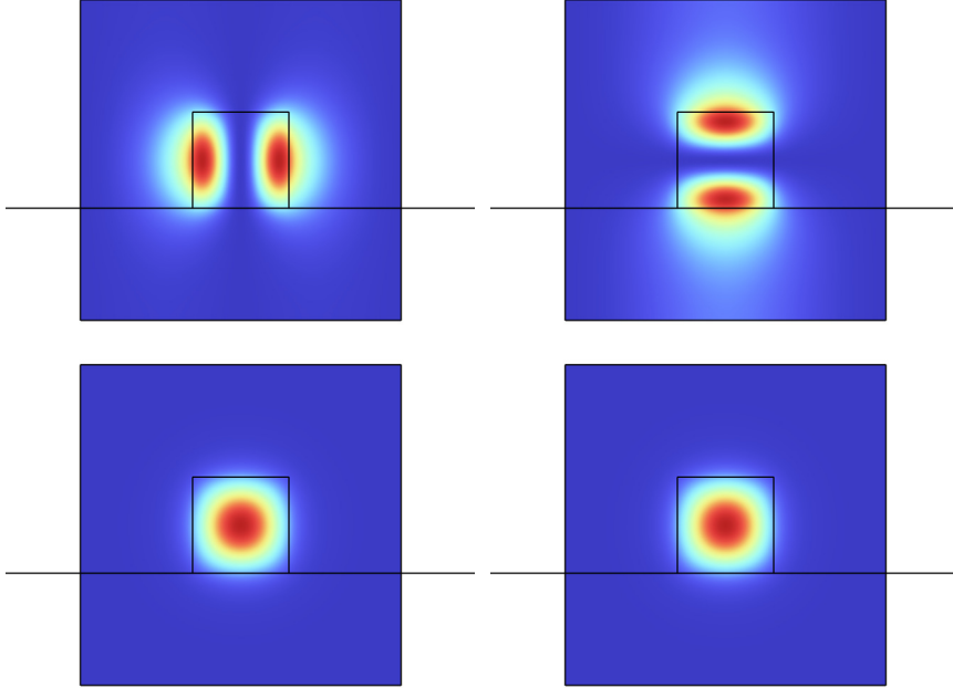
Figure 5: Eigenmodes computed with the stress-optical effect taken into account.
