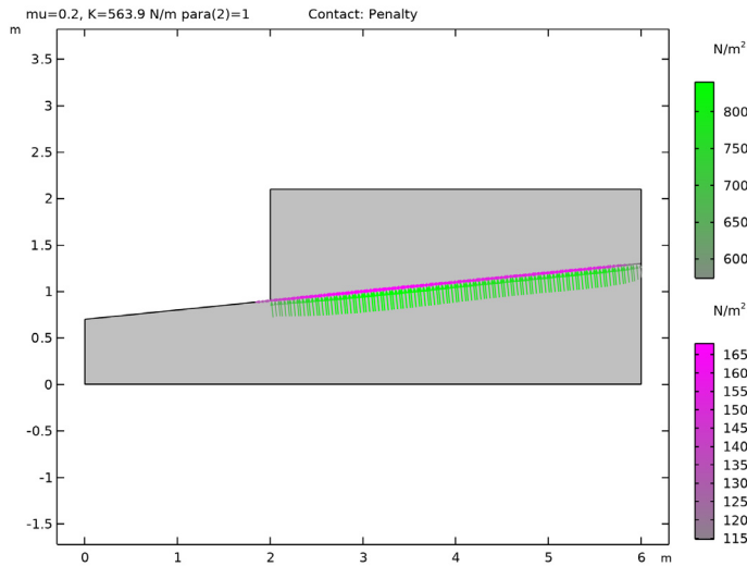
Figure 4: Contact pressure and friction forces acting on the contactor wedge.
