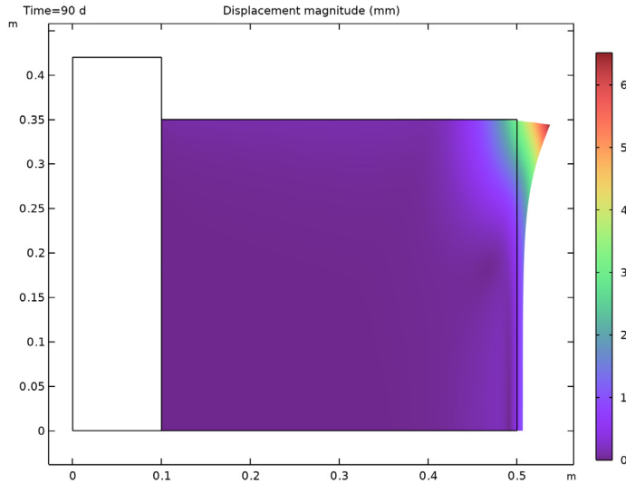
Figure 5: Displacement magnitude and deformation (amplified) after 90 days.
