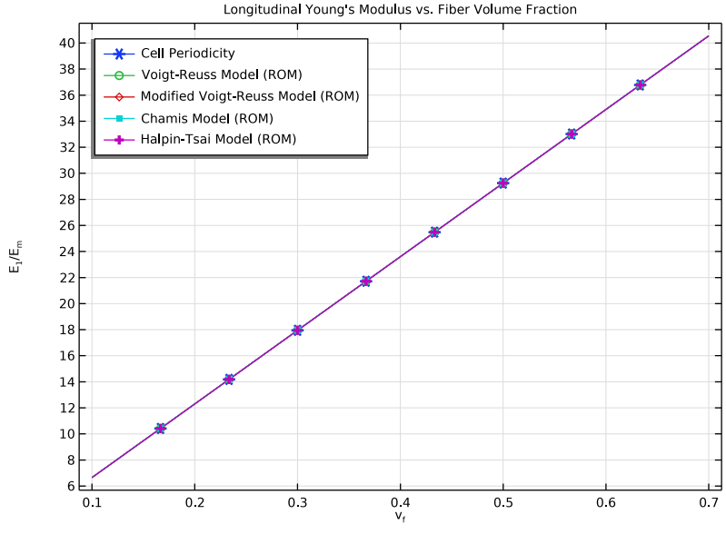
Figure 2: Longitudinal Young's modulus versus fiber volume fraction.
