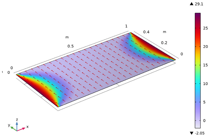
Figure 7: Second principal stress, isotropic material.
