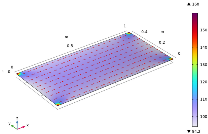
Figure 5: First principal stress, isotropic material.
