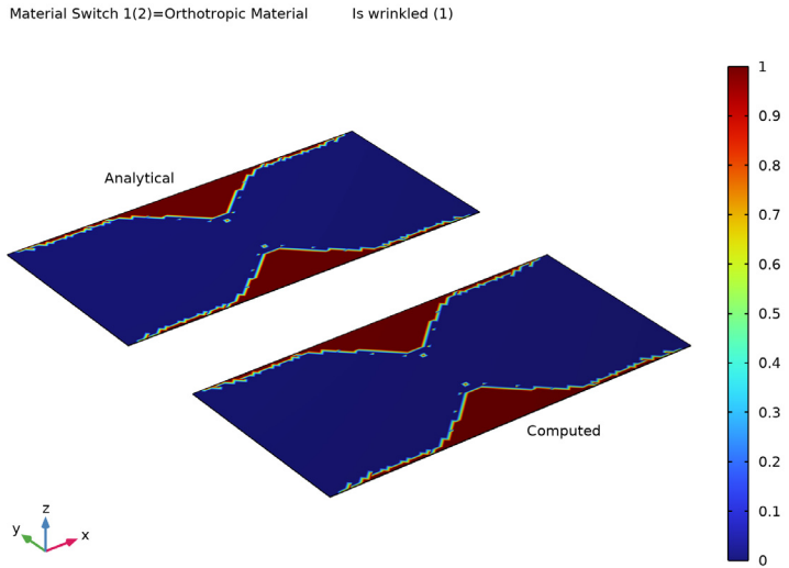
Figure 2: Wrinkled region, orthotropic material.
