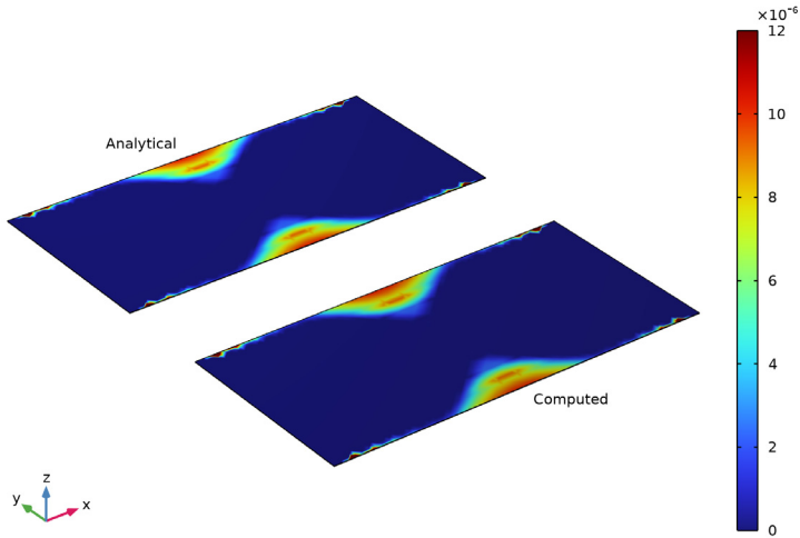
Figure 4: Measure of wrinkling, orthotropic material.
