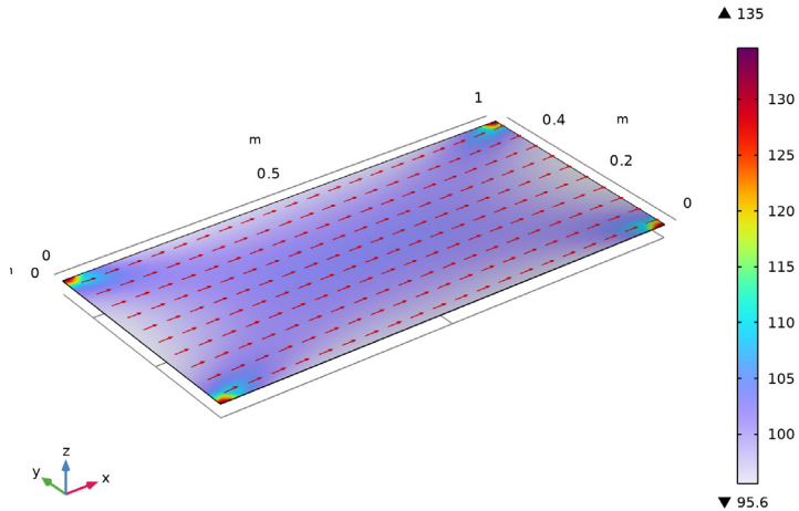
Figure 6: First principal stress, orthotropic material.
