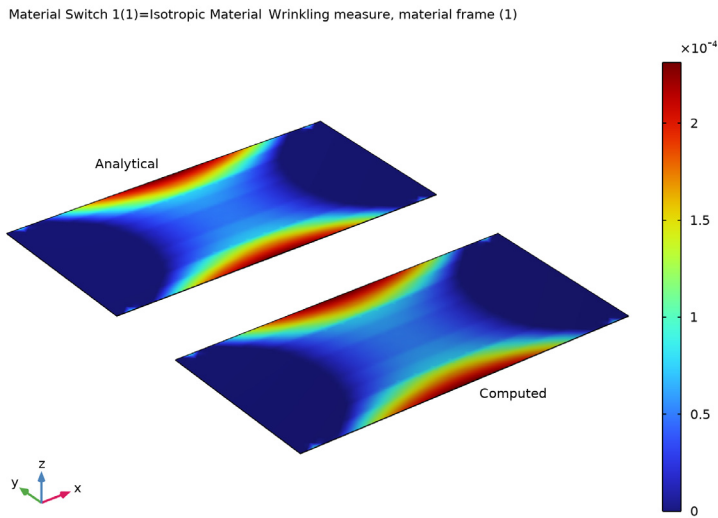
Figure 3: Measure of wrinkling, isotropic material.
