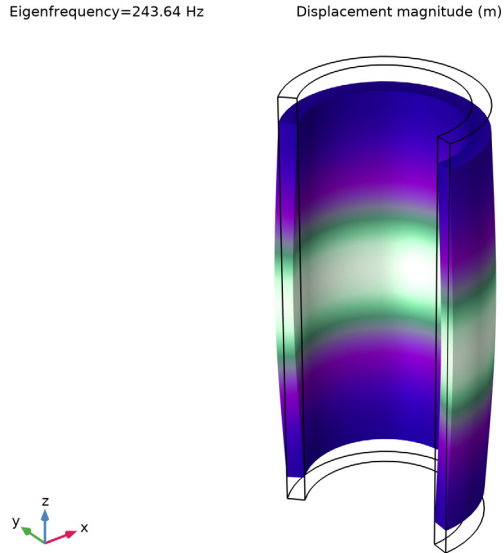
Figure 3: The second nonrigid eigenmode, computed using an axisymmetric shell interface. Due to the offset property, the shell is modeled at the true midsurface, even though the mesh is at the inner boundary of the cylinder.
