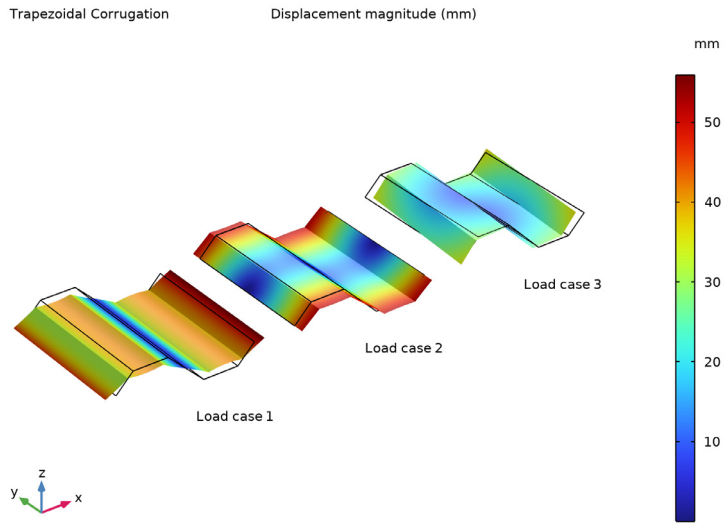
Figure 3: Displacement of the trapezoidal sheet for the translational load cases.
