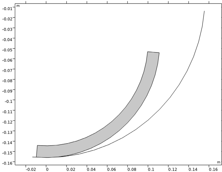
Figure 1: Model geometry.
