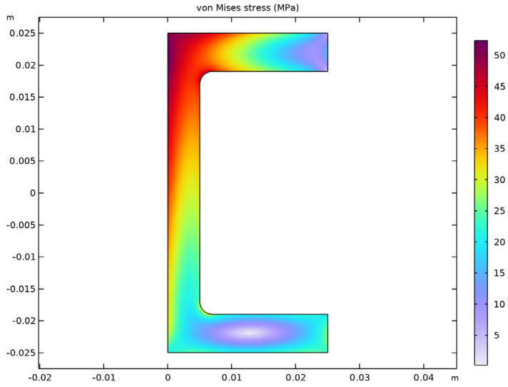
Figure 3: von Mises stress distribution at the fixed end ( x = 0 ).
