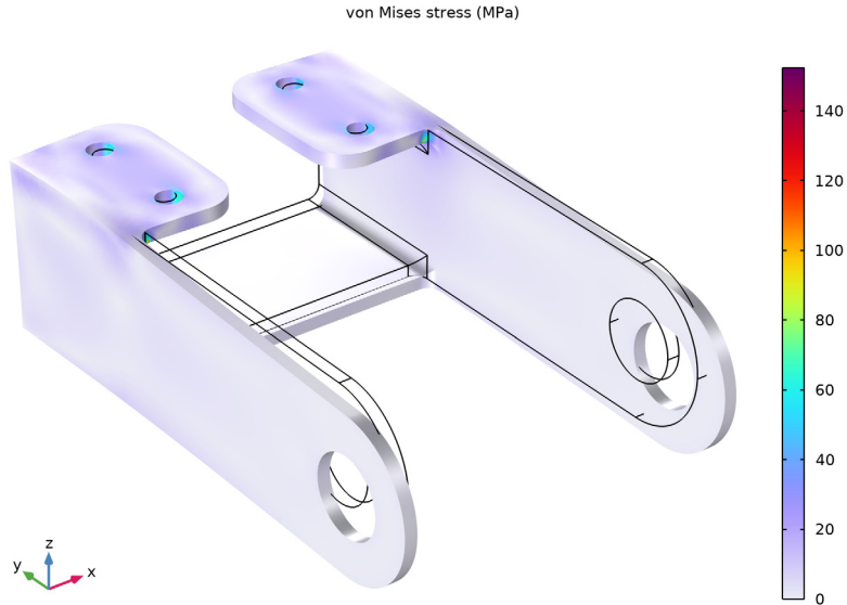
Figure 2: Von Mises stress distribution in the bracket.
