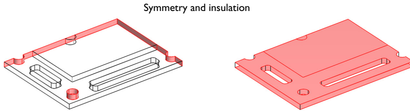
Figure 6: Symmetry and insulation boundaries.
