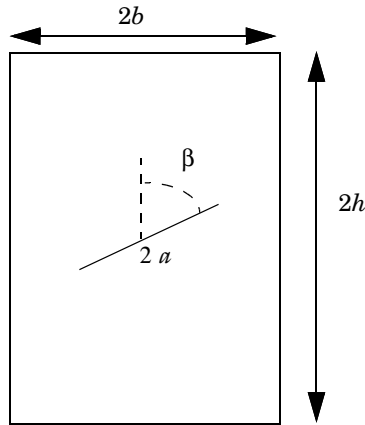
Figure 1: Crack geometry.
