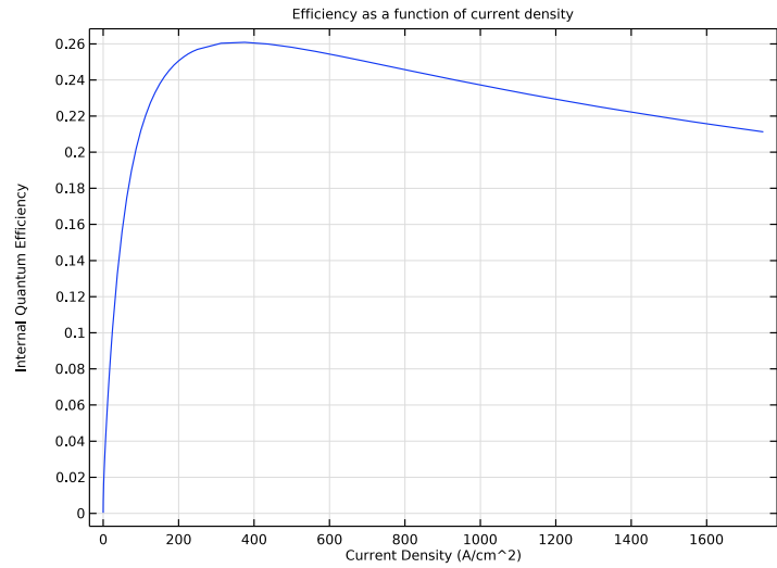
Figure 9: Internal Quantum Efficiency as a function of current density. The rapid decrease for densities above \sim 300 A cm^{-2} limits the current bias which can be applied whilst maintaining acceptable efficiency.
