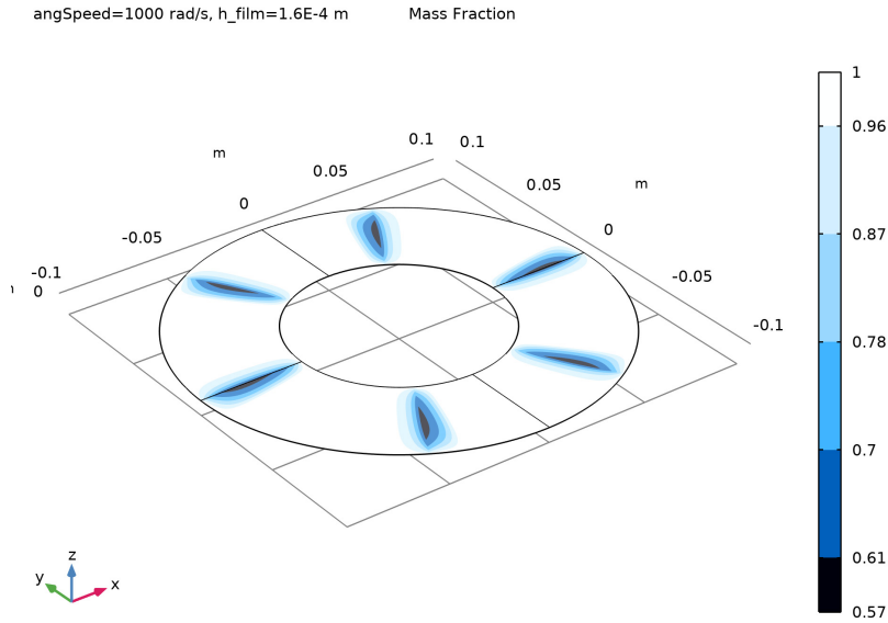
Figure 3: Mass fraction at \Omega = 1000 rad/s with a film thickness of 160 \mu\text{m} .
