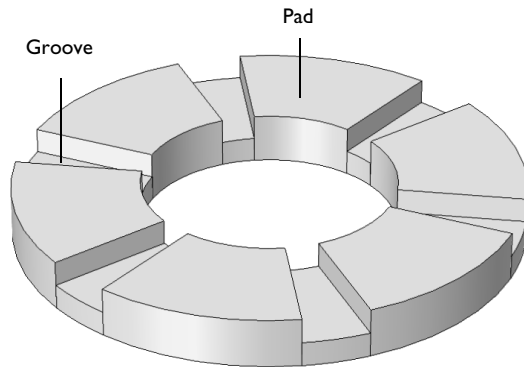
Figure 1: Step thrust bearing geometry.
