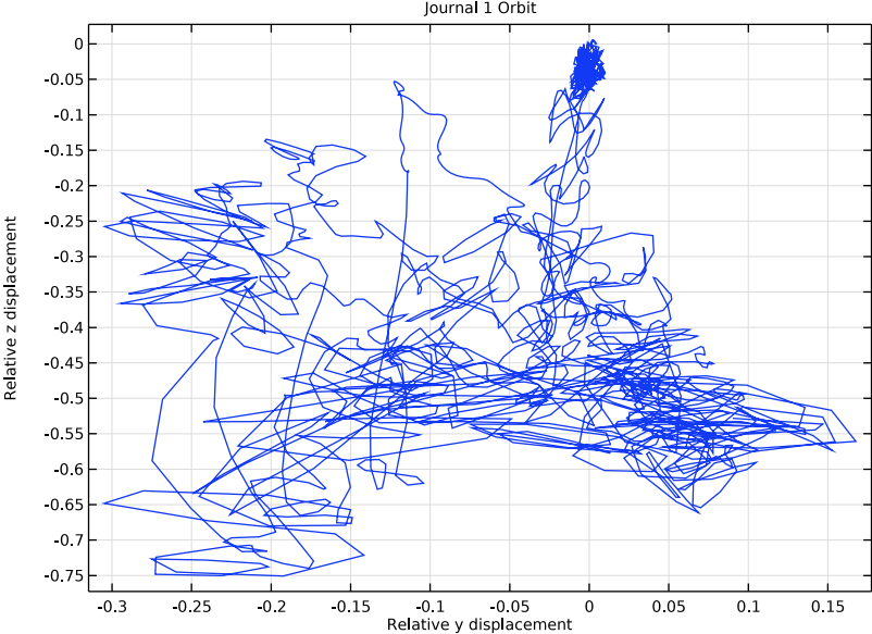
Figure 11: Journal orbit.
