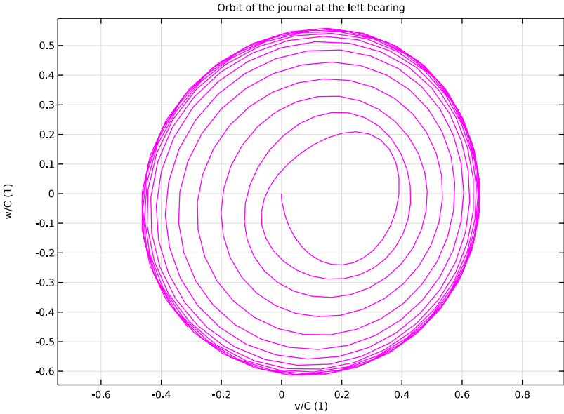
Figure 4: Journal orbit.
