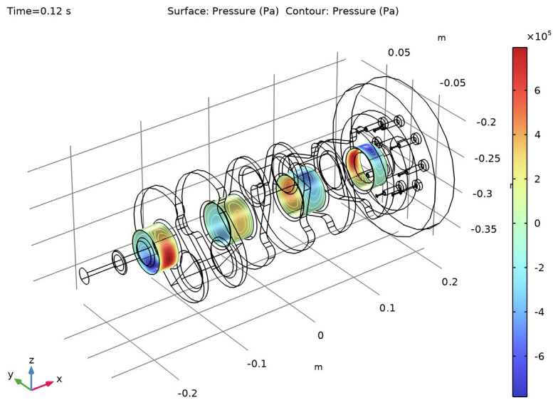
Figure 3: Pressure in the bearings at 0.12 s.
