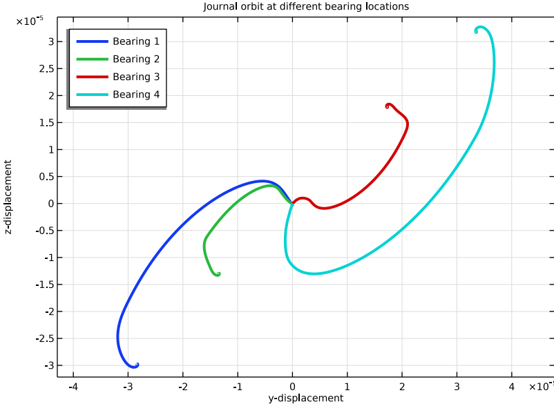
Figure 4: Journal orbits.
