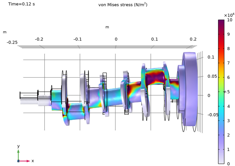
Figure 2: Stress in the crankshaft at 0.12 s.
