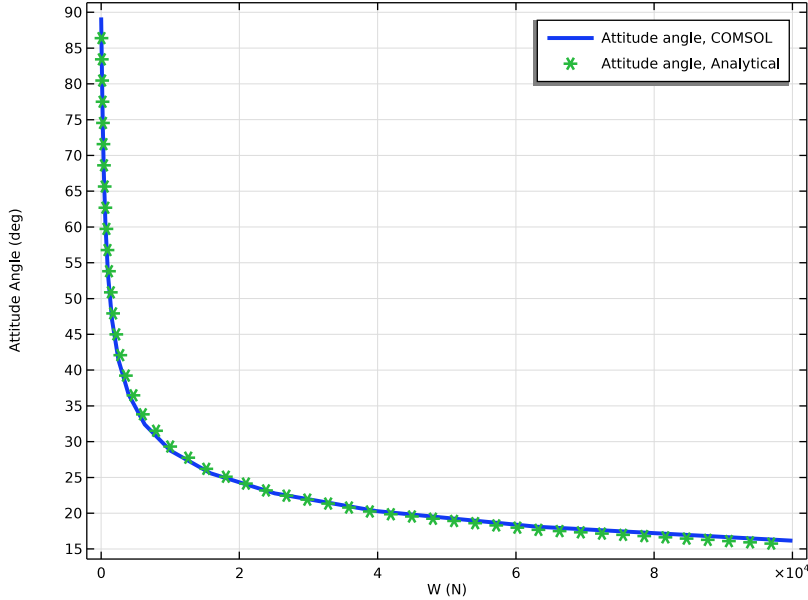
Figure 2: Attitude angle versus load.
