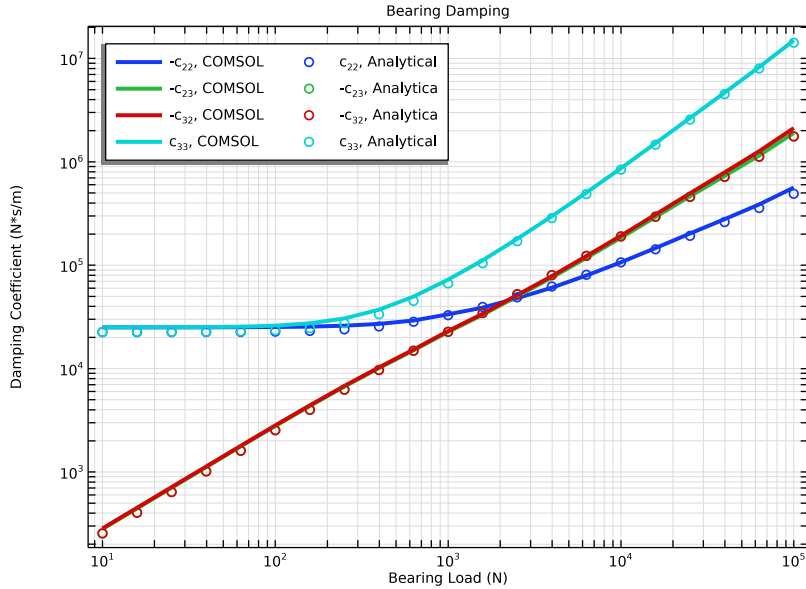
Figure 5: Bearing damping.
