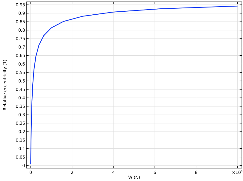
Figure 1: Eccentricity versus load.
