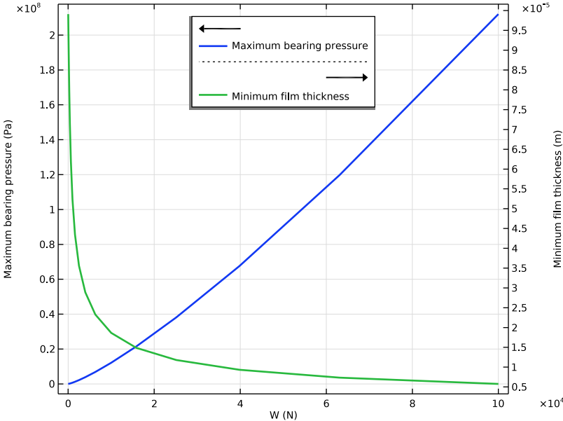
Figure 3: Maximum pressure and minimum film thickness versus load.
