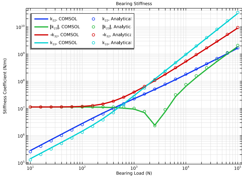
Figure 4: Bearing stiffness.
