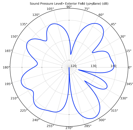
Figure 12: Far-field sound pressure level at a distance of 1m in the yz -plane at 2000 Hz.
