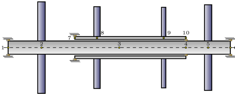
Figure 1: Rotor configuration.
