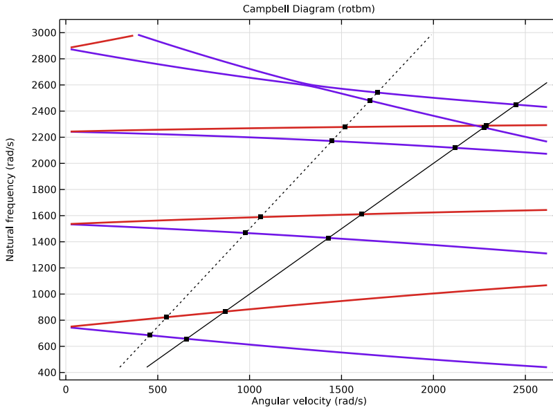
Figure 4: Campbell diagram for the rotor system.
