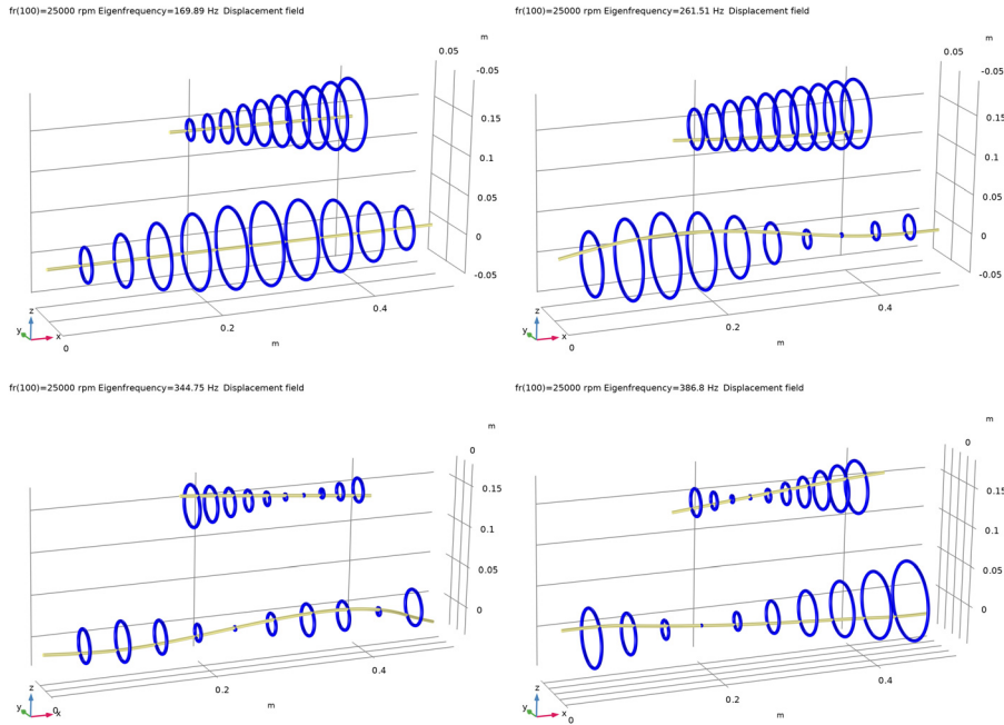
Figure 3: Mode shapes for different frequencies.
