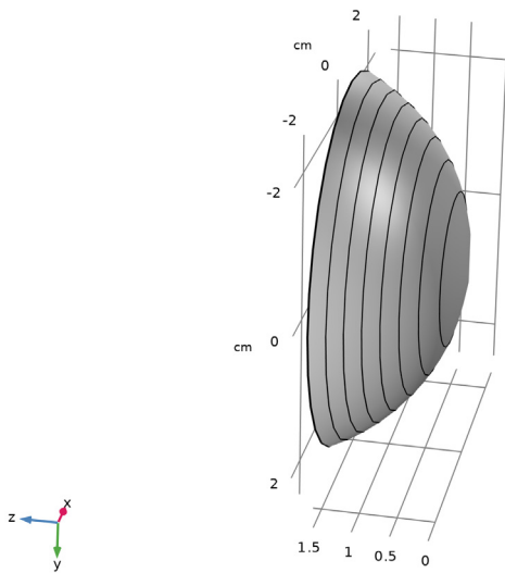
Figure 4: The lens is partitioned by a series of work planes with spacing equal to the desired Fresnel lens thickness.
