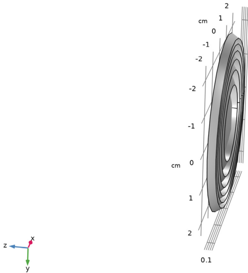
Figure 5: Cylindrical domains are removed from the interior of the lens. The remaining outer rings are moved to the same plane to form a flat Fresnel lens.
