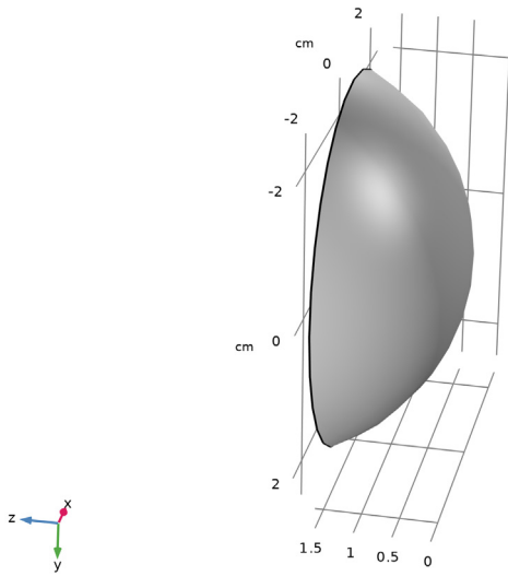
Figure 3: A plano-convex lens imported from the Ray Optics Module Part Library. When the focal length is short, the lens is very thick.
