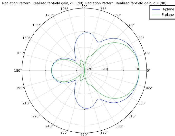
Figure 4: Polar plot: E-plane and H-plane patterns.
