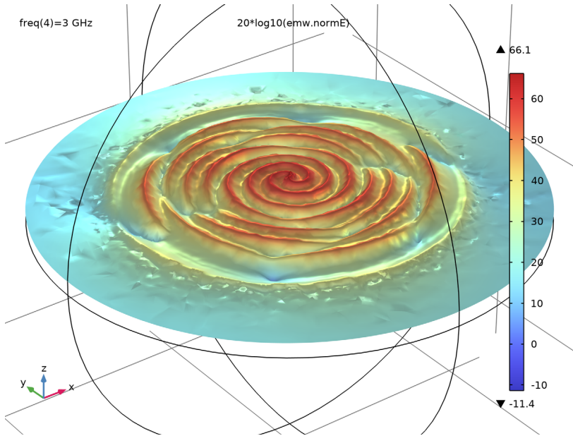
Figure 2: The log-scaled electric field norm on the xy -plane describes how the electric fields are confined on a slotted substrate.
