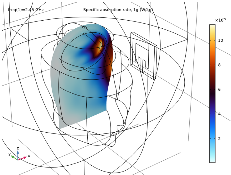
Figure 3: The above slice plot shows the SAR for 1g of mass.
