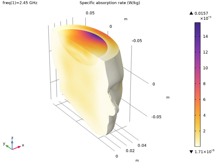
Figure 2: The computed local SAR values are visualized for a part of the head using a filter subfeature. The brain part closest to the radiating antenna has the highest SAR values.
