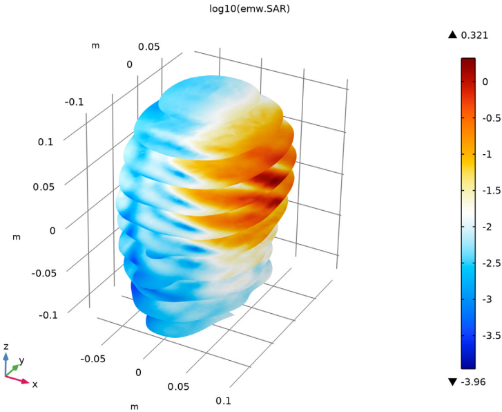
Figure 2: Log-scale slice plot of the local SAR value.
