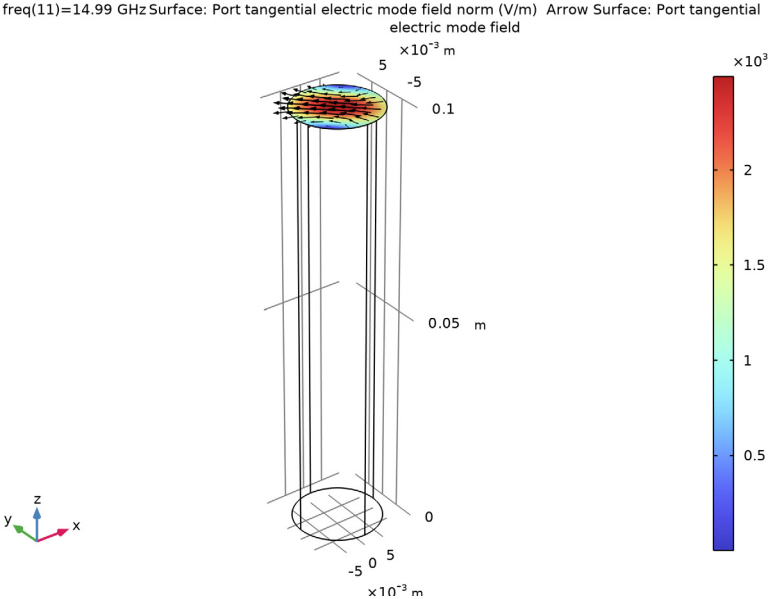
Figure 2: The first TE_{11} mode of the outpost.
