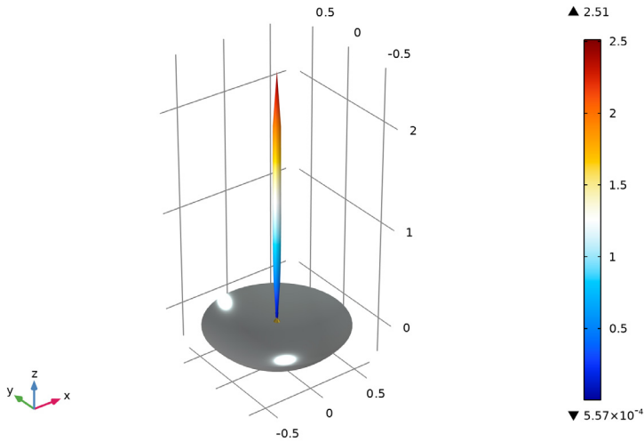
Figure 3: The very sharp 3D far-field radiation pattern is visualized over the axial feed circular horn and parabolic reflector.
