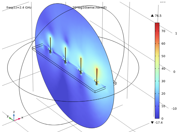
Figure 2: The strongest electric fields are observed around the excited monopole antenna. The plot also shows that the excited energy is coupled to other antennas elements.
