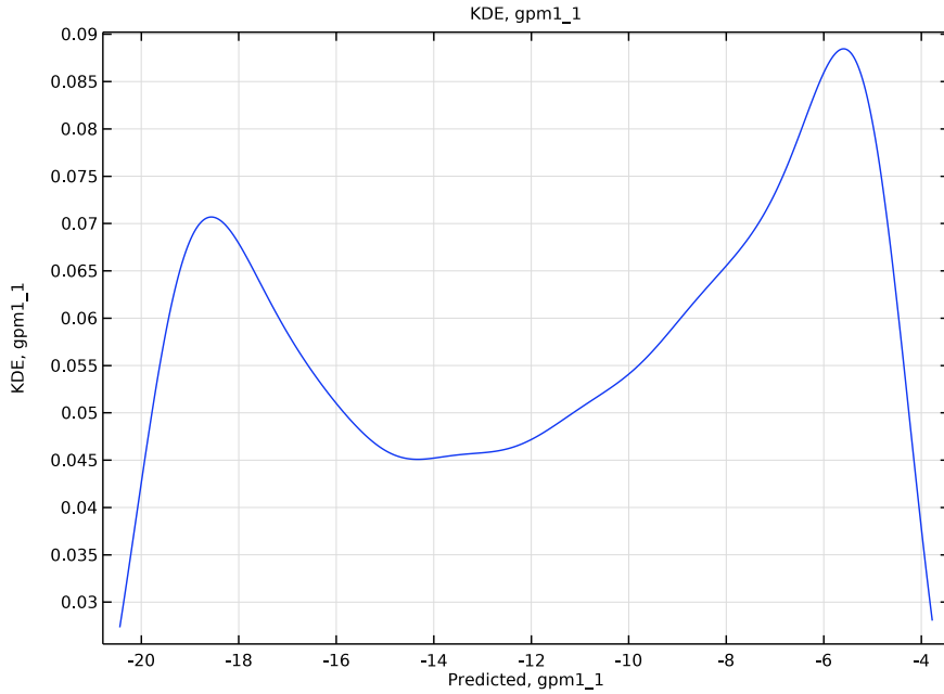
Figure 4: Kernel density estimation (KDE) illustrating the probability density function of the Q_{oI} .
